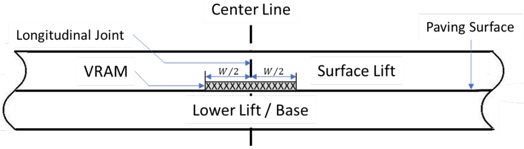
Figure 1: Example to illustrate VRAM application. Drawing not to scale. Cross sections will vary. Refer to plans.
