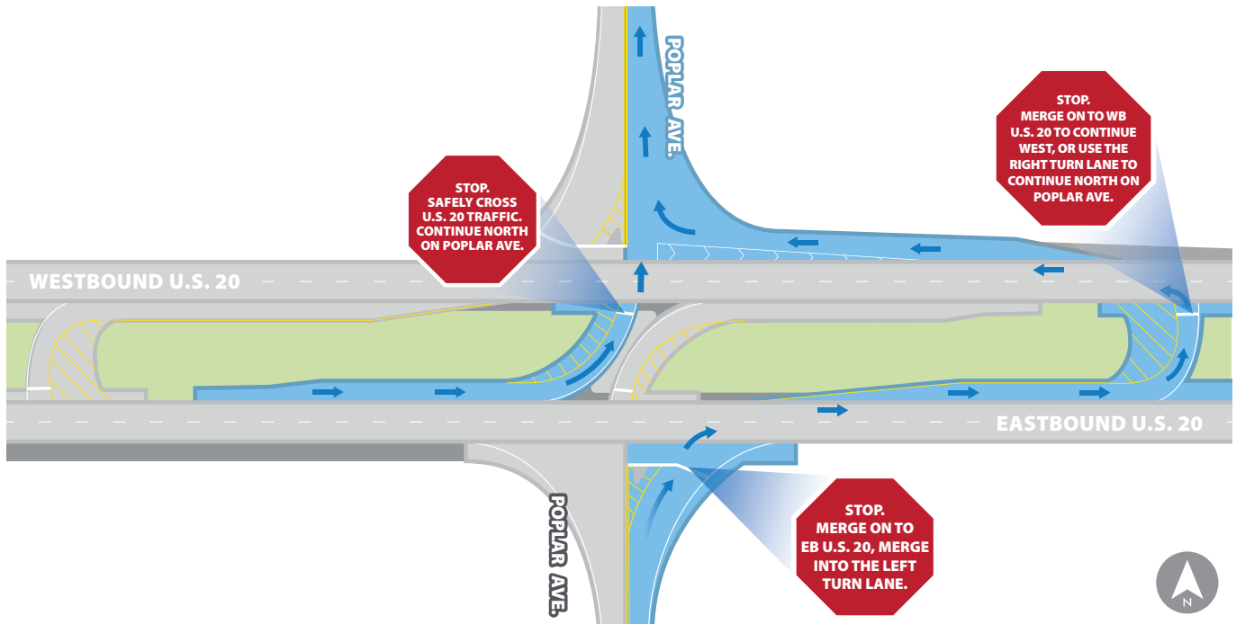
Figure 5.3: Reduced-conflict interchange (Example shows the reduced-conflict interchange at U.S. 20 and Poplar Ave. in Webster County)
